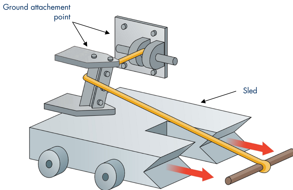
Figure A1 – Configuration générale du dispositif d'essai Figure A1 – General definition of the apparatus
