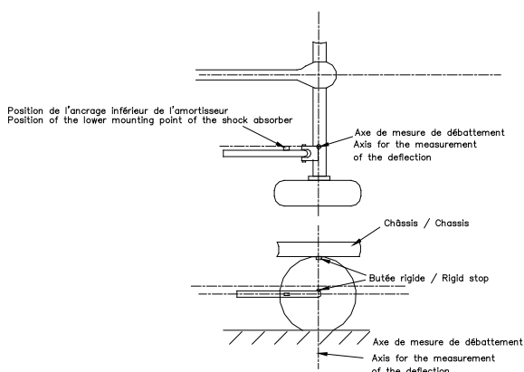
Dessin / Drawing 287-11
