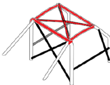
Dessin / Drawing 253-68
