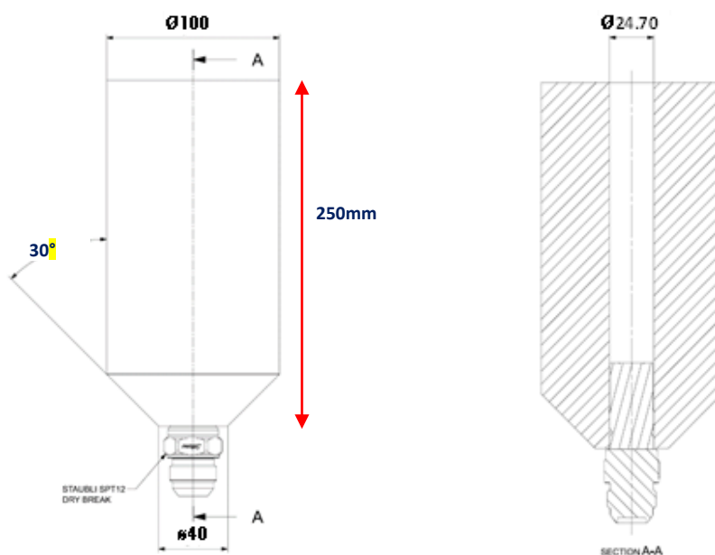
Dessin / Drawing 283-01
