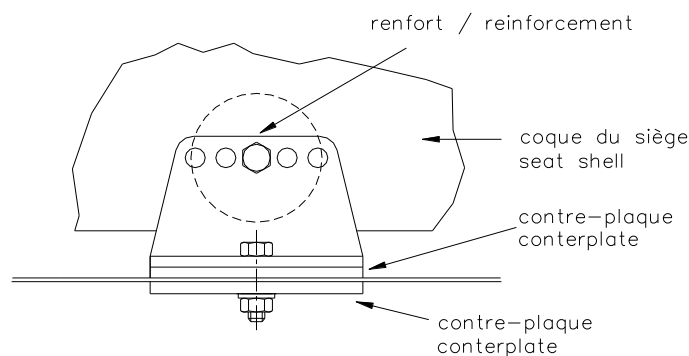
Dessin / Drawing 253-65
