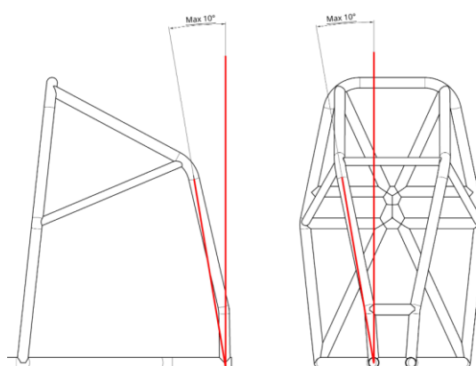
Dessin / Drawing 279B-15
