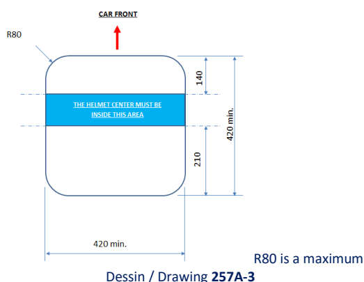
Dessin / Drawing 257A-3
