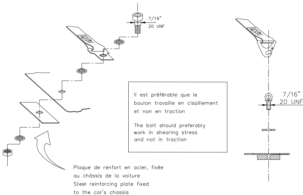
Dessin / Drawing 253-62
