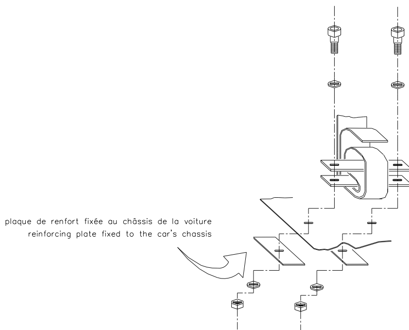
Dessin / Drawing 253-64
