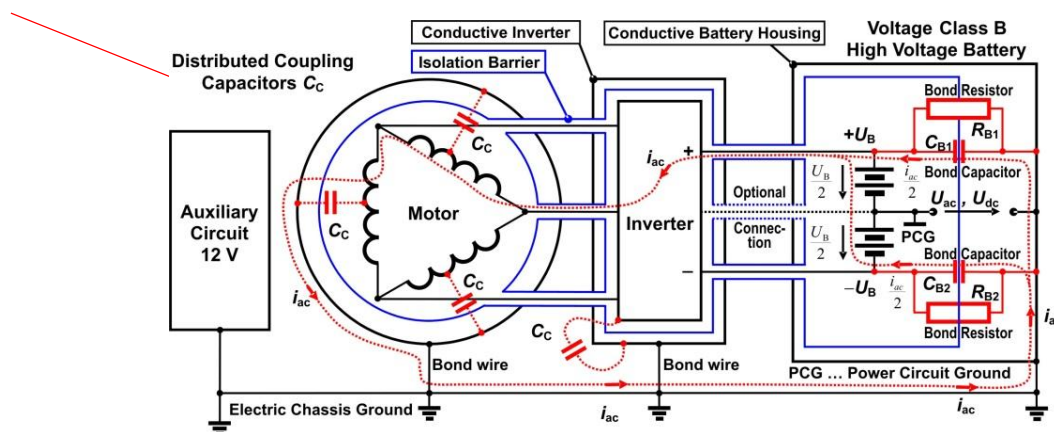
Dessin 6 / Figure 6
