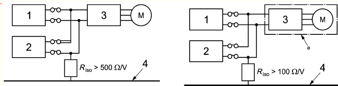
Dessin 7 / Figure 7
