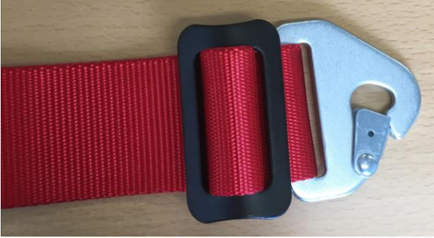
ALTERNATIVE ATTACHMENT - CROTCH STRAP (2X ANCHOR PLATES - 24E0050)
