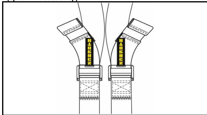
A2-4) Position / Position : 2" left pelvic adjuster (opt. release strap) pull-down or pull-up configurations
