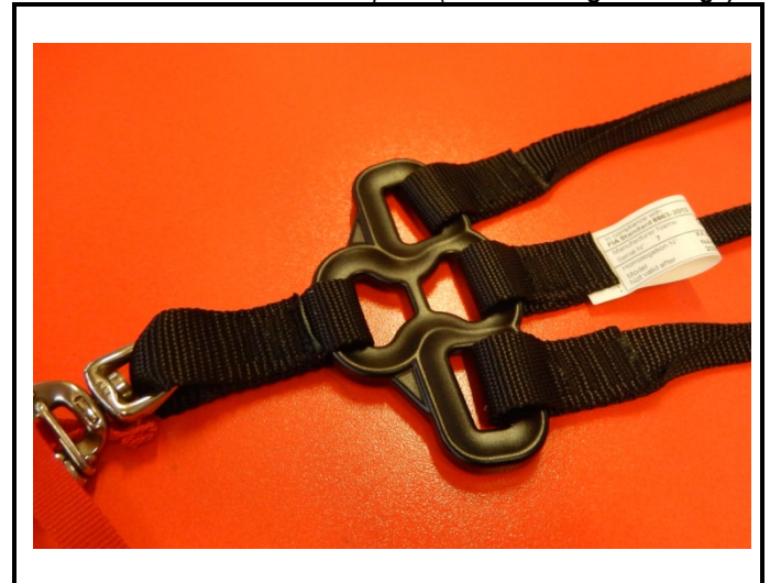
A6) Autre hardware - photo 3/4 avant Other hardware - 3/4 front photo (front webbing anchorage)
