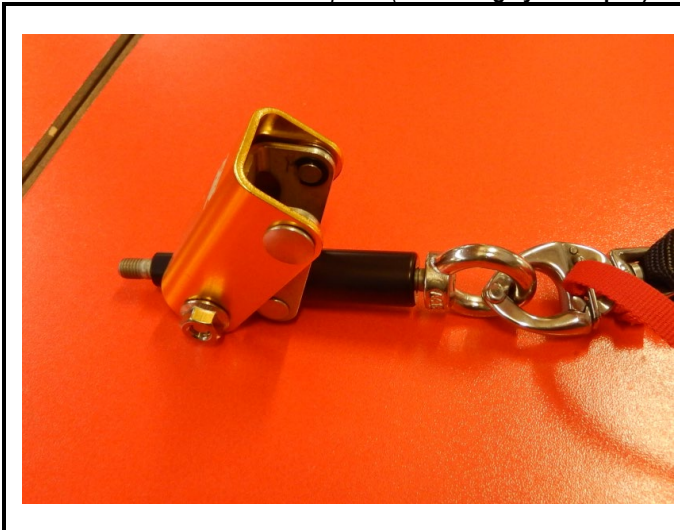
A5) Autre hardware - photo 3/4 avant Other hardware - 3/4 front photo (tensioning system open)
