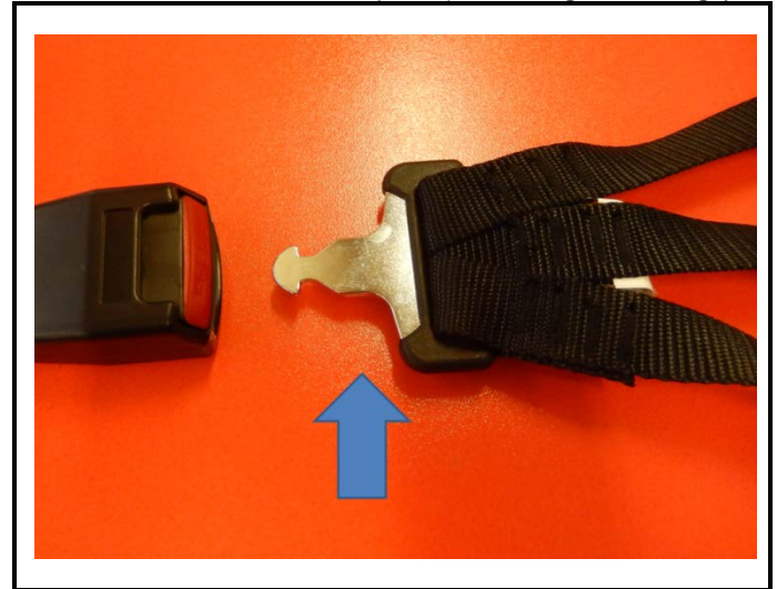
A6) Autre hardware - photo 3/4 avant Other hardware - 3/4 front photo (front triangle anchorage)
