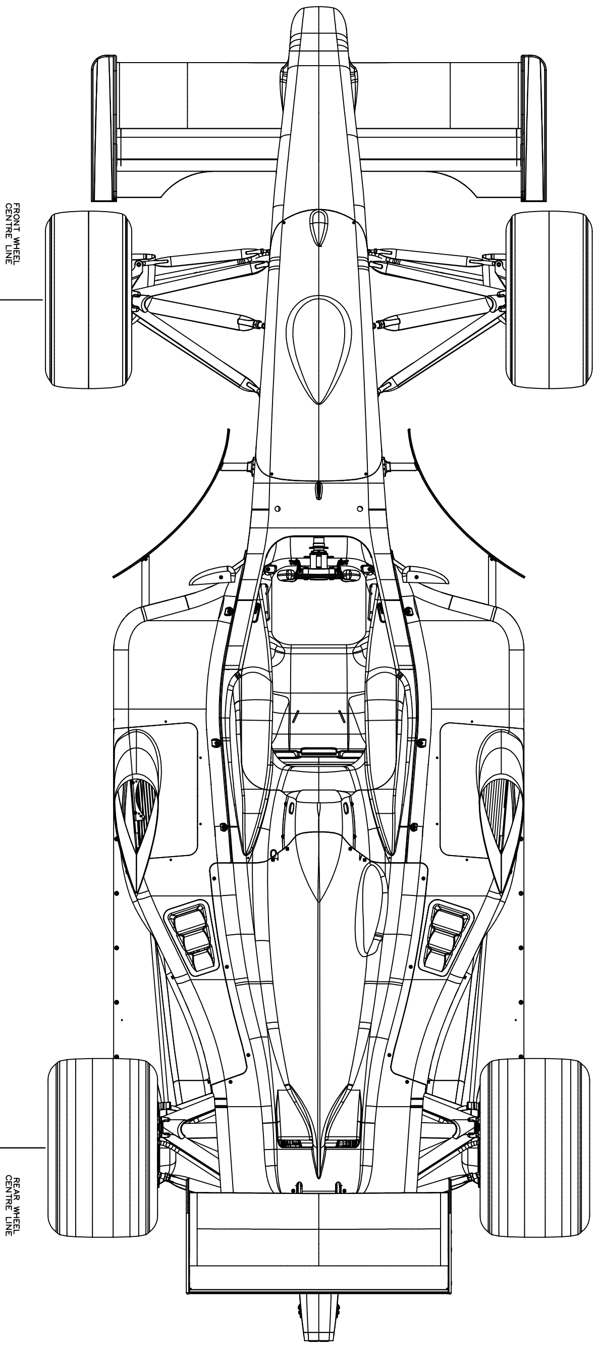
MEASUREMENT HOLES IDENTIFIED BELOW - 6 PLACES
