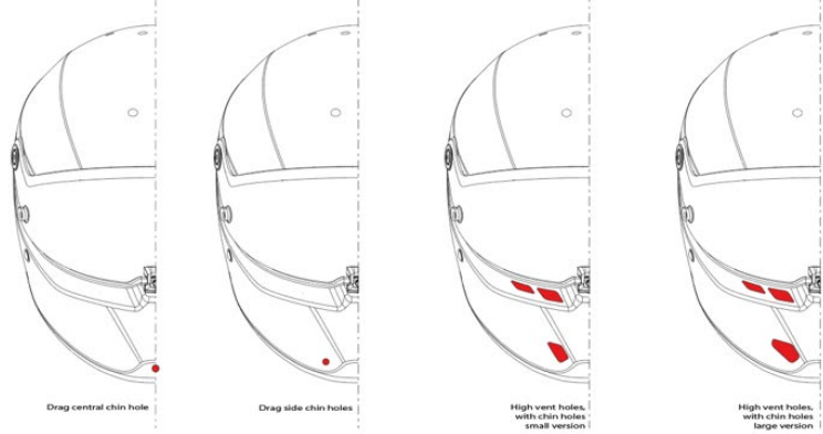
Chin ventilation holes (optional)
