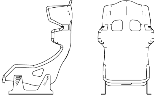
Seat Name: HGT EVO Seat p/n: HA0-0906 Brackets p/n: HA0-0954 Setup position n°1
