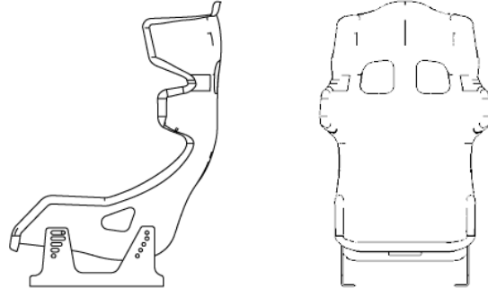
Seat Name: HGT EVO Seat p/n: HA0-0906 Brackets p/n: HA0-0954 Setup position n°2
