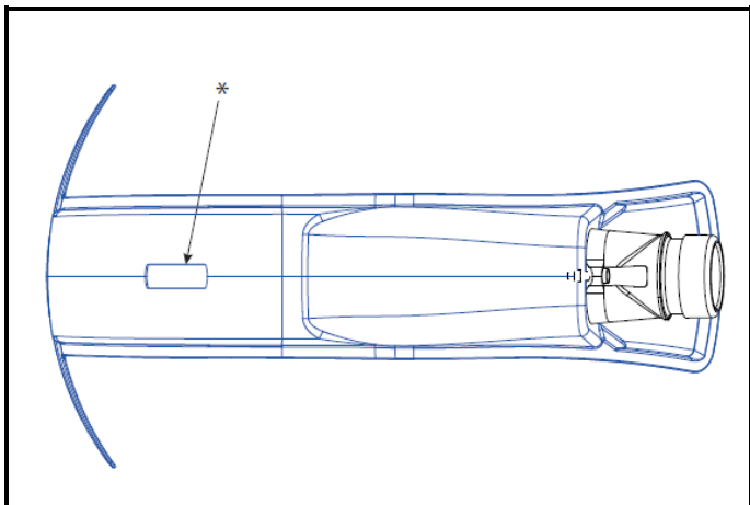
E11) modular top-air connector 0° with improved assembly system for long air-cap
