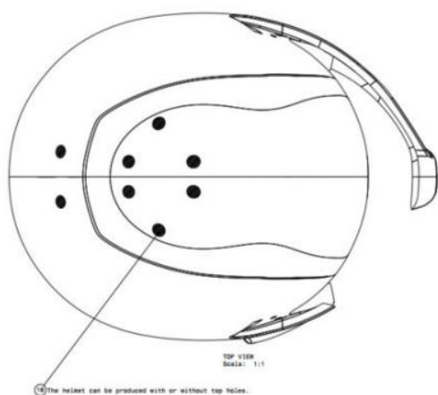
SHELL VENTILATION HOLES - optional
