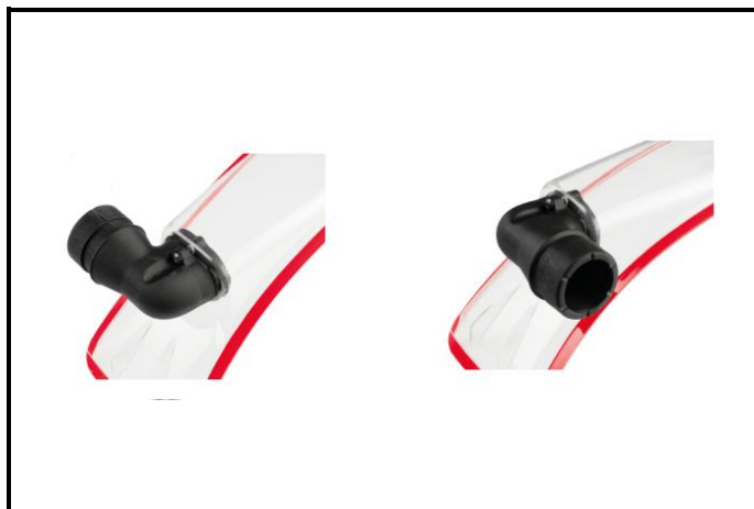
E9) modular top-air connectors 90° with improved assembly system for short air-cap
