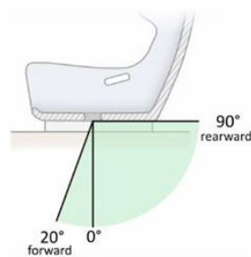
Dessin / Drawing 253-61
