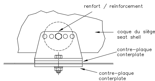
Dessin / Drawing 253-65
