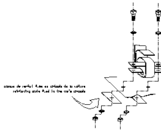
Dessin / Drawing 253-64
