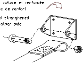
Dessin / Drawing 253-63
