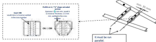
Construction "C"
