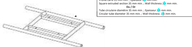
Construction "D"
