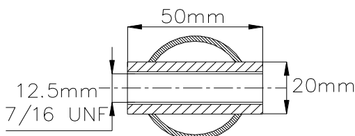
Dessin / Drawing 253-67
