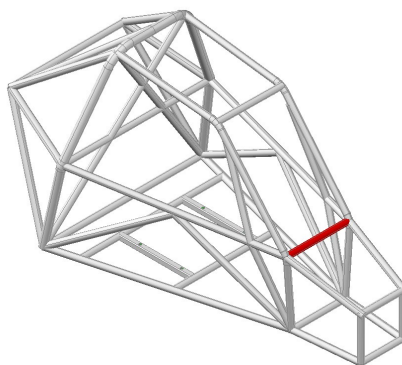
Dessin / Drawing 279A-12
