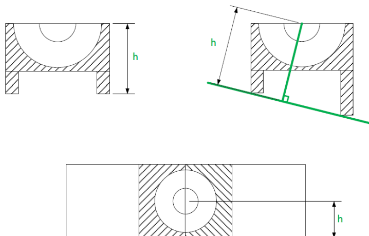
Dessin/Drawing 2
