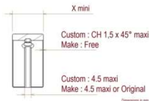
Dessin/Drawing 4
