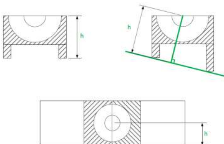
Dessin/Drawing 2
