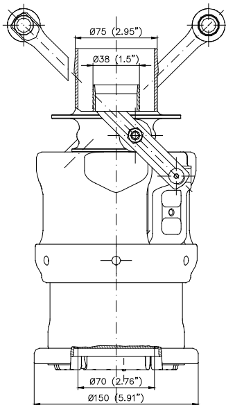
Coaxial
