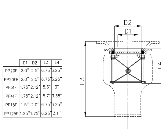
Prise femelle / Push pull series female
