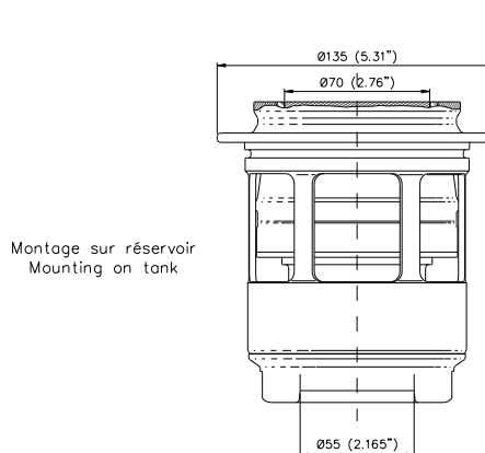
Female Coupling
