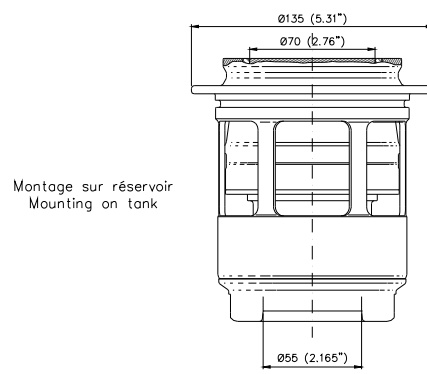
Female coupling
