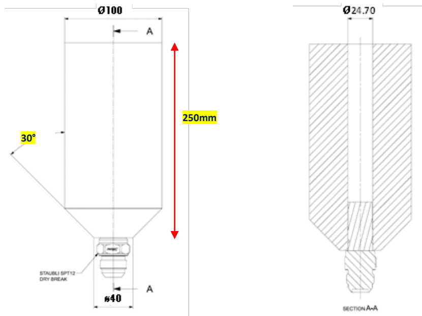
Dessin / Drawing 283-01
