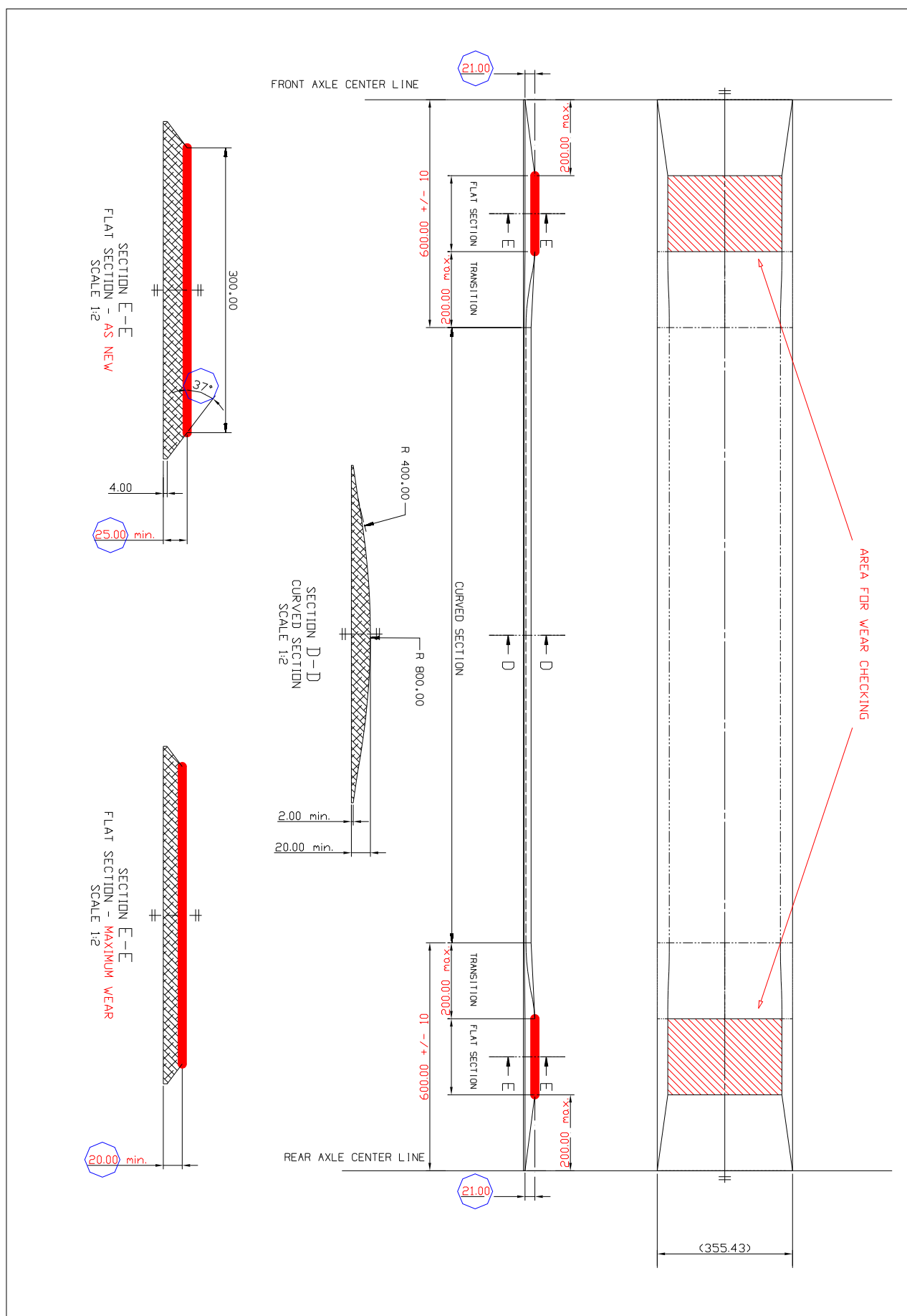
Dessin / Drawing 2
