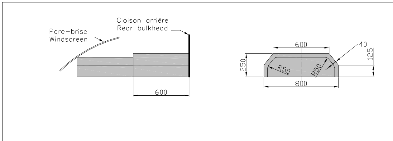
Dessin / Drawing 4
