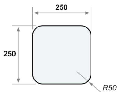
Drawing 1.2
