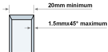
Drawing 2.5
