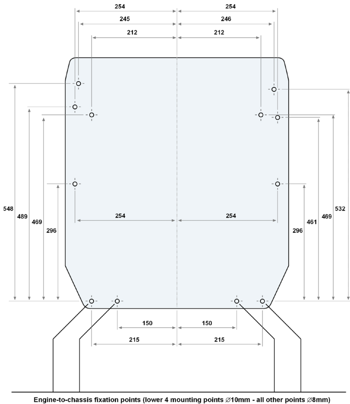
Drawing 2.1
